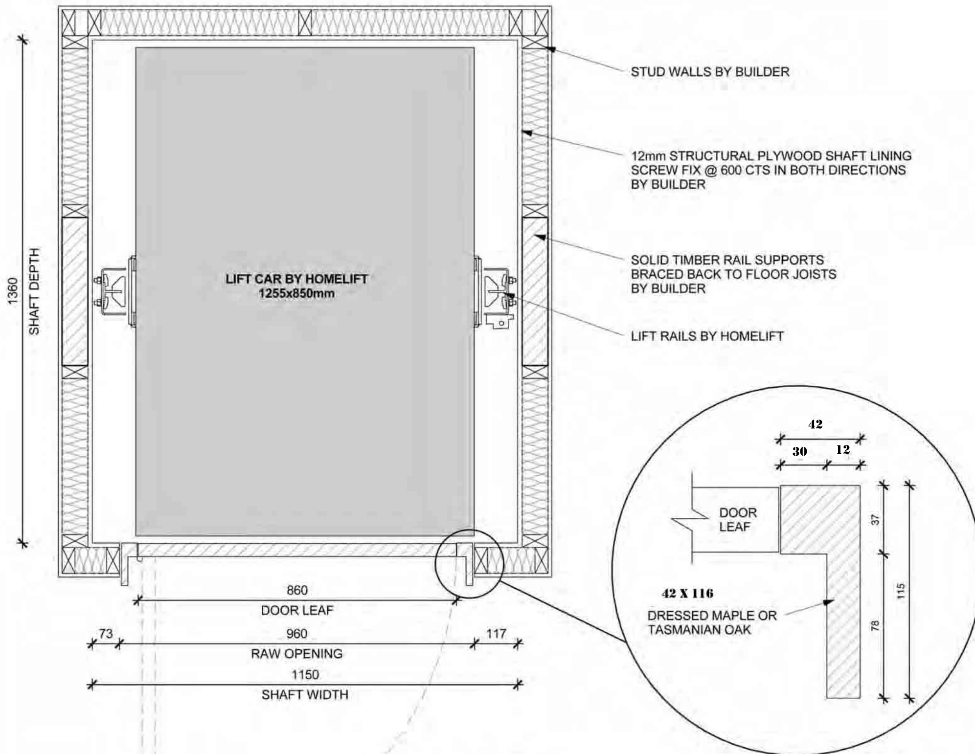
PLAN OF LIFT CAR scale: 1:10 @ A3
