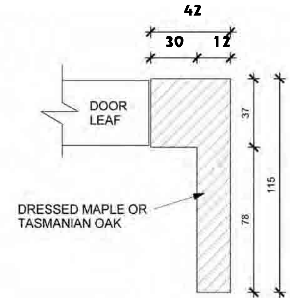
DOOR JAMB / FRAME PROFILE scale: 1:2 @ A3
